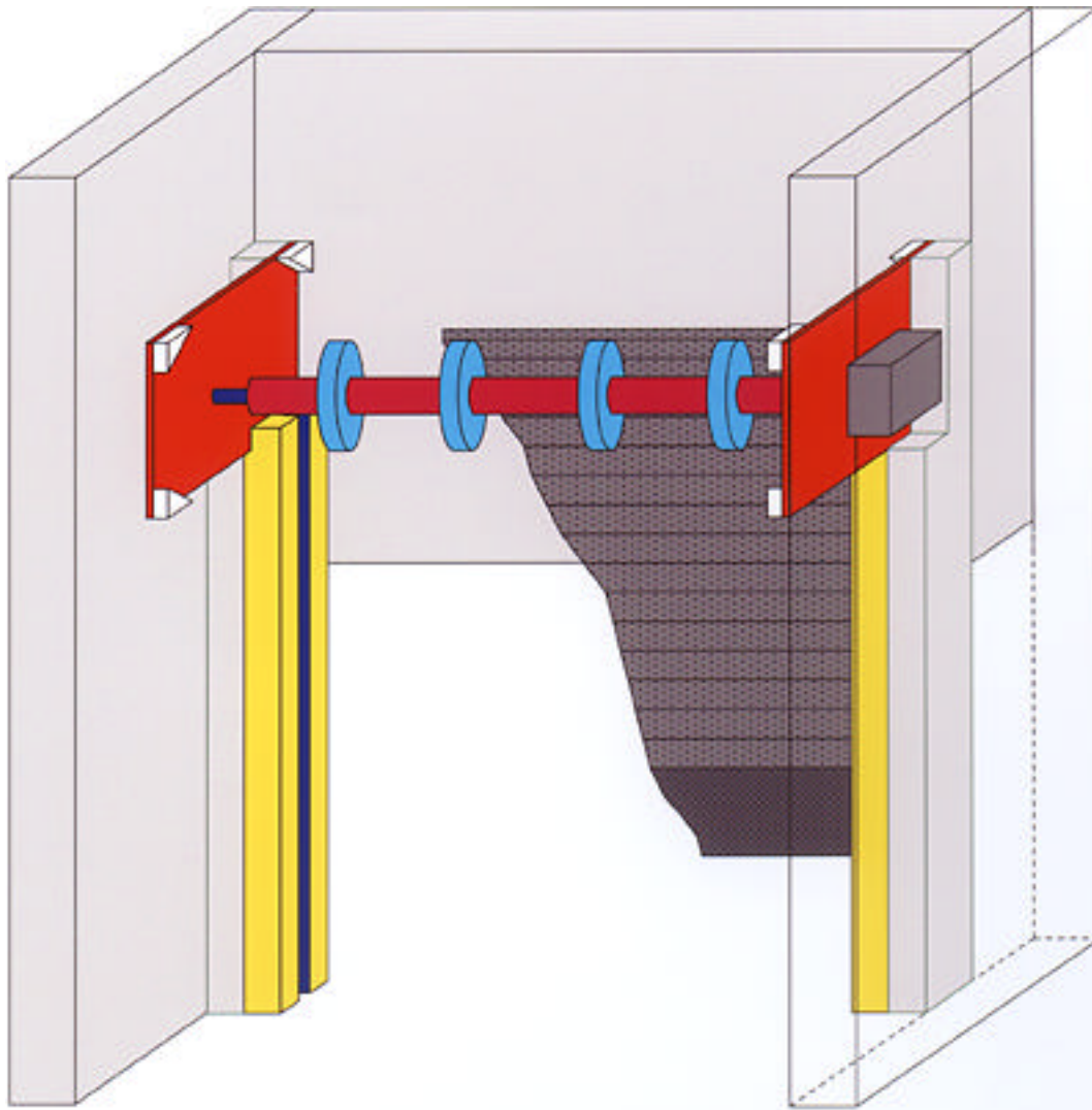
Between Wall Mount On Face of Lintel With Pack Outs (Shown Without Hood)
